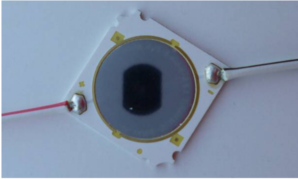
Figure: Alignment of the cable to solder pad LES10 and LES15
