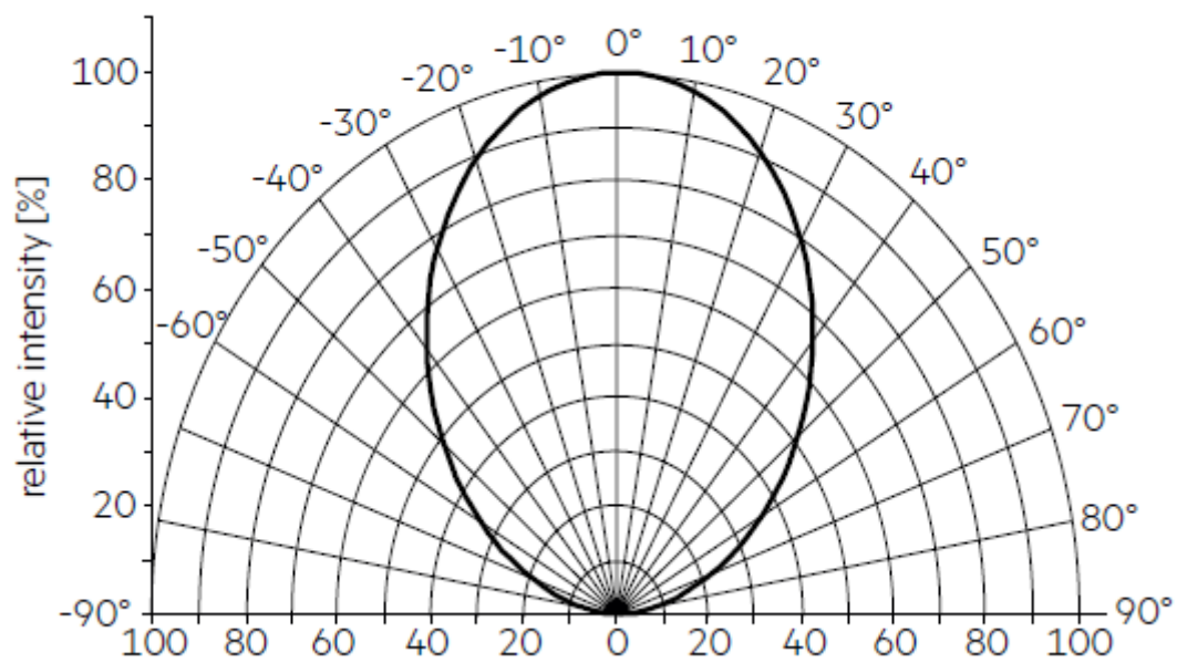
Light distribution with housing
