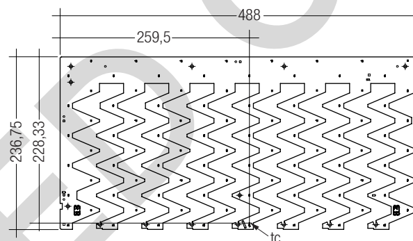
QLE G4 488x237mm 2500lm ADV
