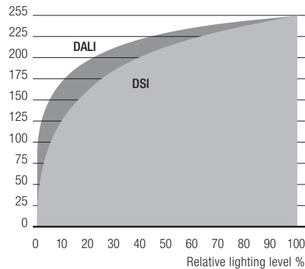
Dimming characteristics as seen by the human eye
