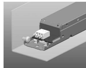
Screw M4, screw head diameter 8–10 mm
