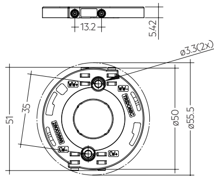
Housing with LES13
