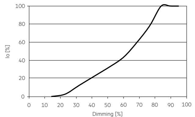
4.1.6 Phase cut dimming curve (depends dimmer) Output current vs dimming
