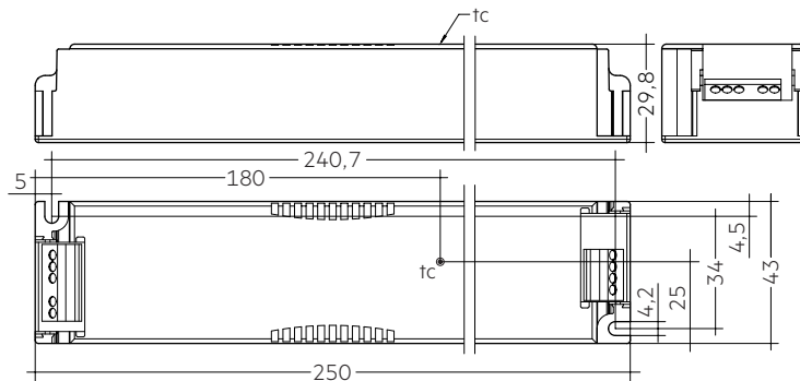
Without strain-relief
